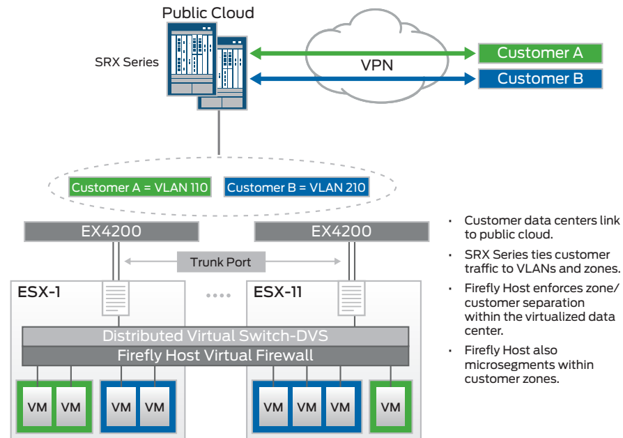
Figure 5: Multi-tenancy management and isolation enforcement.
